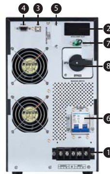
Titan Vista Neo P 6KS/10KS (Back View)
